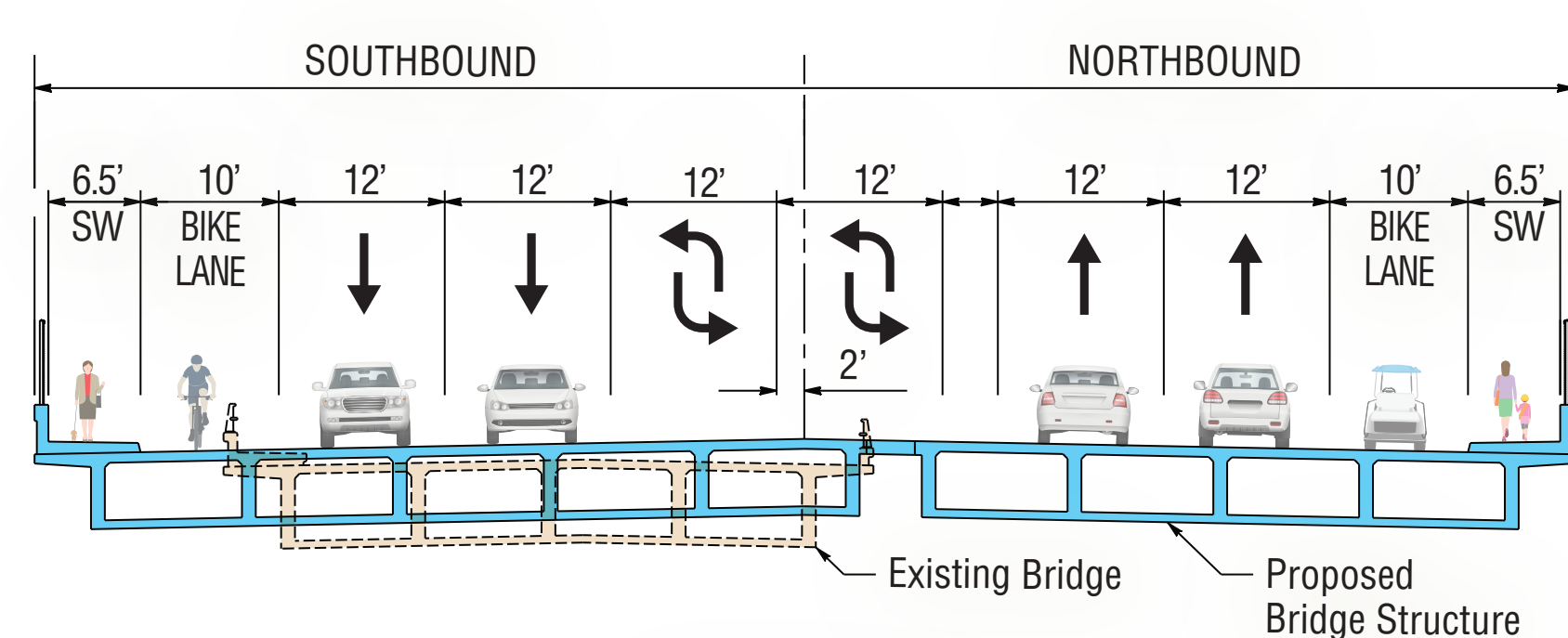
SECTION A-A Monroe Street Overcrossing (I-10)
