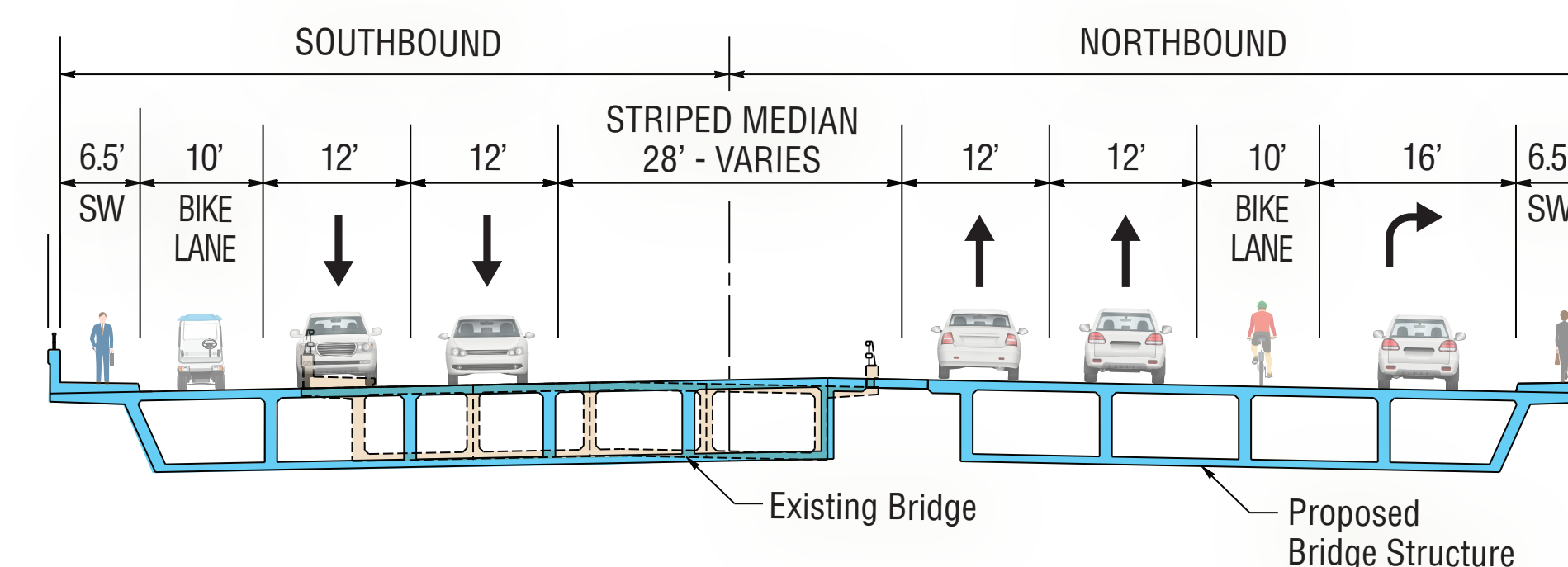
SECTION B-B Monroe Street Channel Bridge
